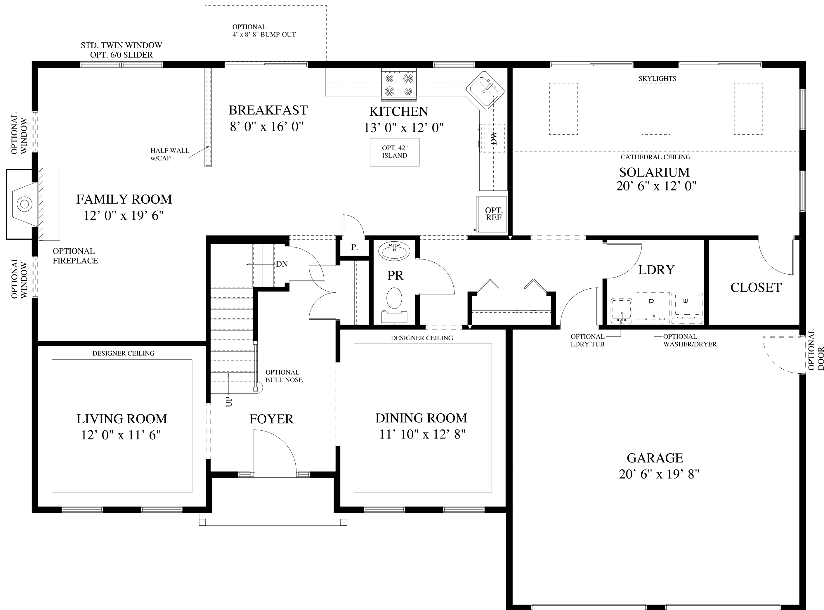
STD. FIRST FLOOR PLAN - SOLARIUM
